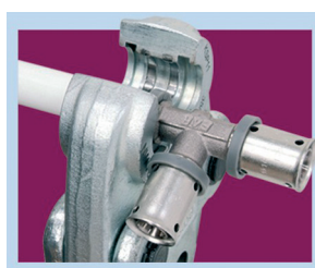
MACHOIRES TH
